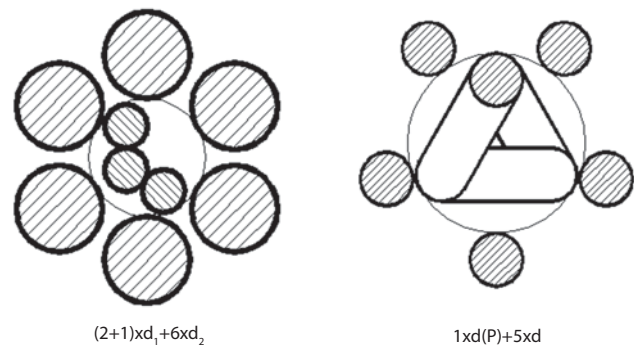
Fig. 5. Steel cord constructions with rubber complete penetration and an improved fixation of core's wires (P – preformed)
