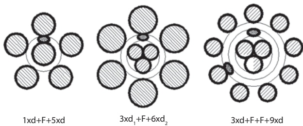
Fig. 8. Separation ply between wires in multiple ply constructions
