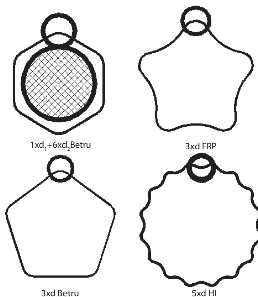
Fig. 3. New steel cord constructions providing complete penetration of rubber mixture are cord “Betru”(Bekaert total rubber penetration) and “FRP” (Full rubber penetration), and also “HI” (High Impact)
