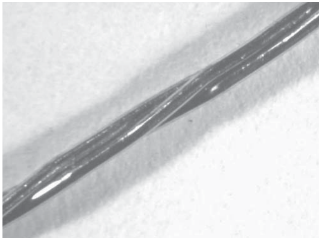
Fig. 4. Steel cord appearance 3x0,30 HT FRP
