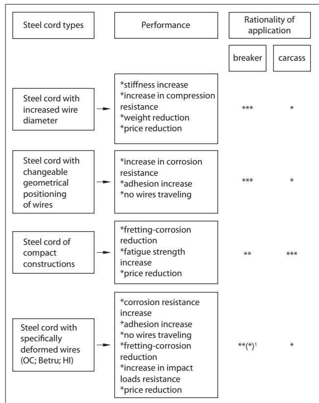
Fig. 1. Distribution chart of modern steel cord types (* – normally is not desirably; ** – possible; *** – very efficient; 1 – HI only as a screening ply)
