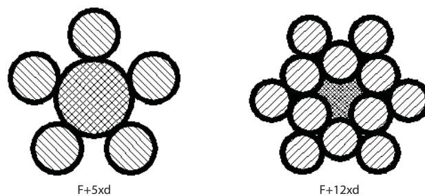
Fig. 6. Constructions of combined steel cord (F- fiber)
