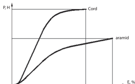
Fig. 7. Diagram of aramid core extension together with twisted steel cord
