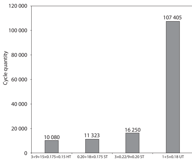
Fig. 2. Relative data for cycle quantity undergone by steel cord in a rubber free condition at tests for 3-roller bending with load of 20 % from breaking strength
