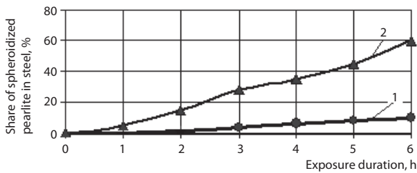
Fig. 3. A share of spheroidized pearlite in steel (%) after medium (line 1) and high (line 2) tempering depending on exposure duration (hours)
