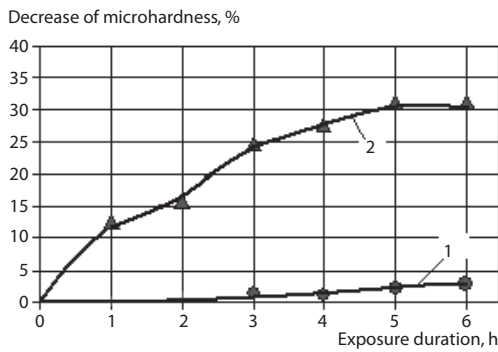
Fig. 2. Influence of exposure duration (hours) at medium (line 1) and high (line 2) tempering on microhardness decrease (%) of studied steel
