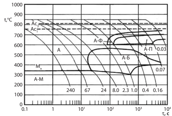
Fig. 4. Continuous cooling transformation diagram of quality carbon steel, containing 0.39 % C; 1.08 % Cr and 0.25 % Mo
