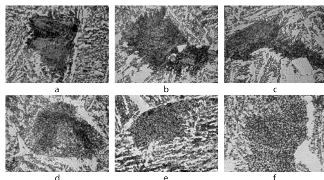
Fig. 1. Microstructure of (x 800) chromium-molybdenum steel: a - initial condition and after medium (b, c) and high (d-f) tempering with exposure of 1 hour (d), 3 hours (b, e) and 6 hours (c, f) with subsequent air cooling (a-b, d-e) or in the furnace (c, f)
