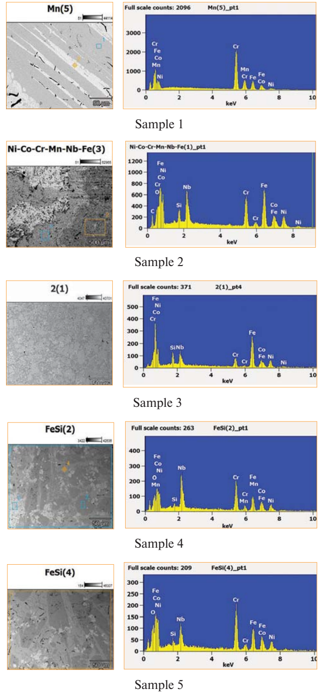
Fig. 3. Structure of pilot alloys
