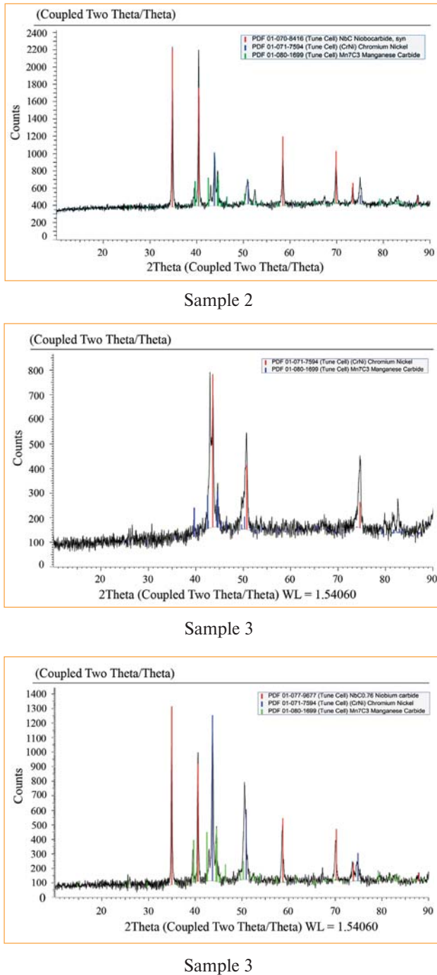
Fig. 2. The results of X-ray phase analysis for pilot samples with different niobium content
