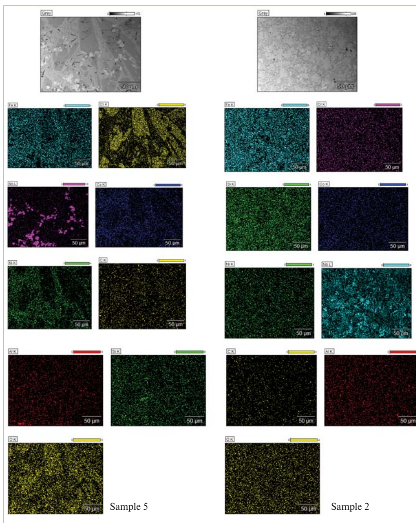
Fig. 4. The chart of elements distribution in the samples 2 and 5
