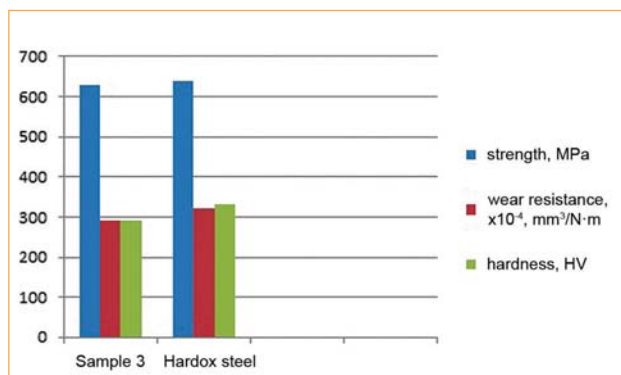
Fig. 5. Comparative diagram of properties of the pilot alloy and steel
