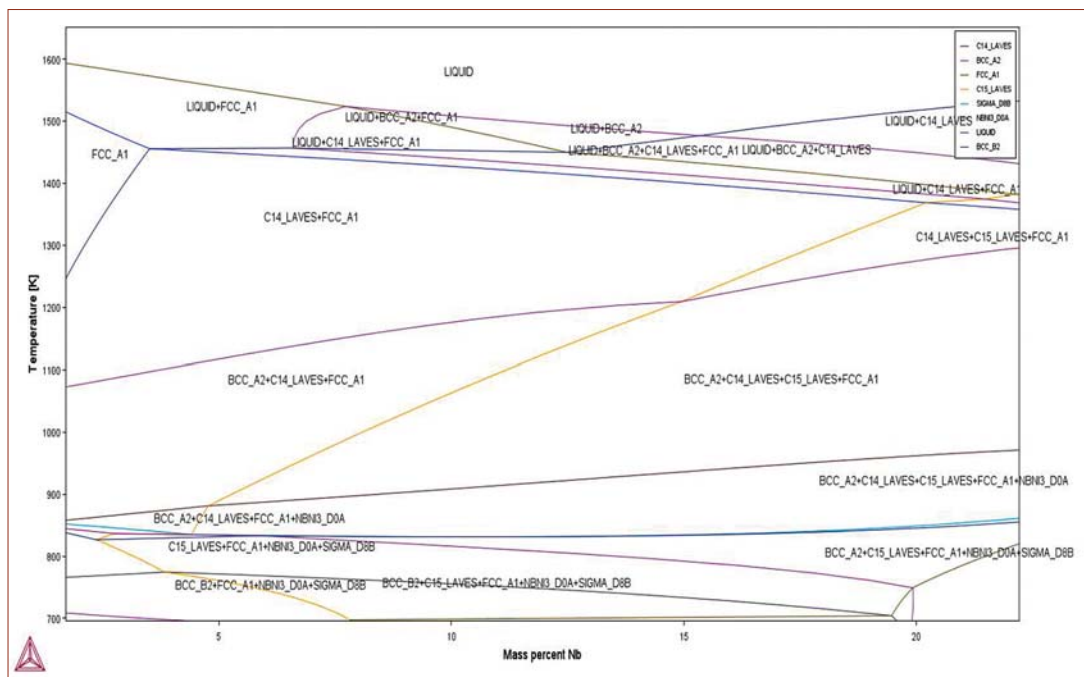
Fig. 1. Equilibrium diagram for alloys of the Cr–Mn–Ni–Fe–Co–Nb system, which is calculated ThermoCalc software
