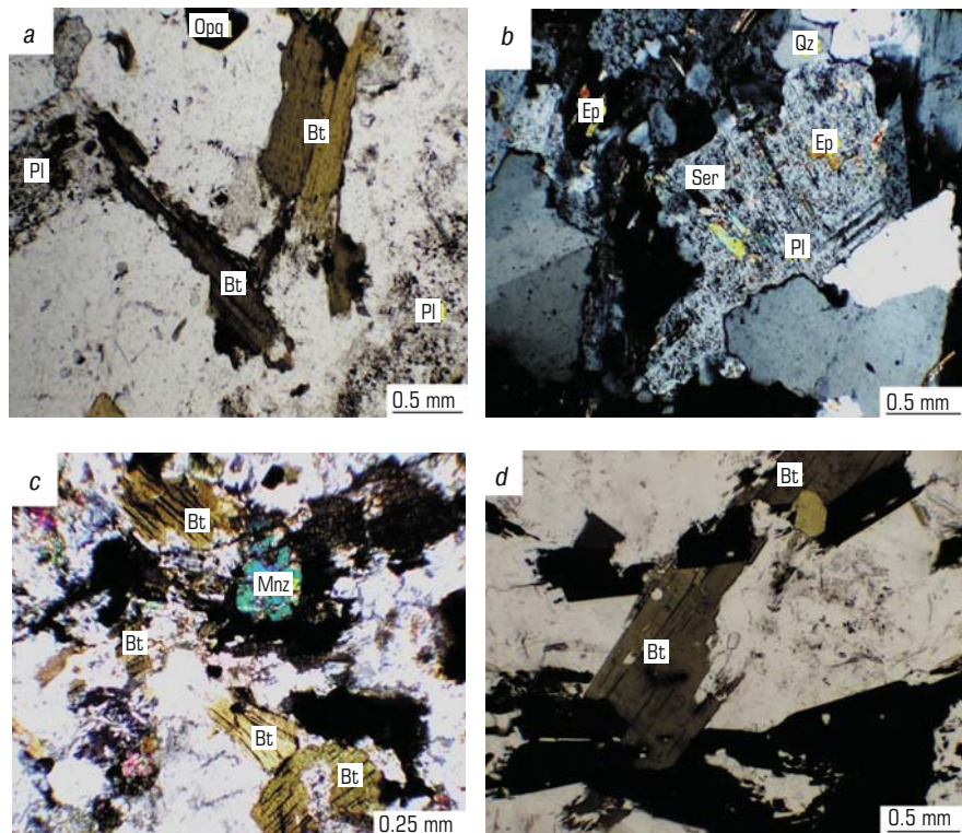
Fig. 2. Microimages of granites and diorites
