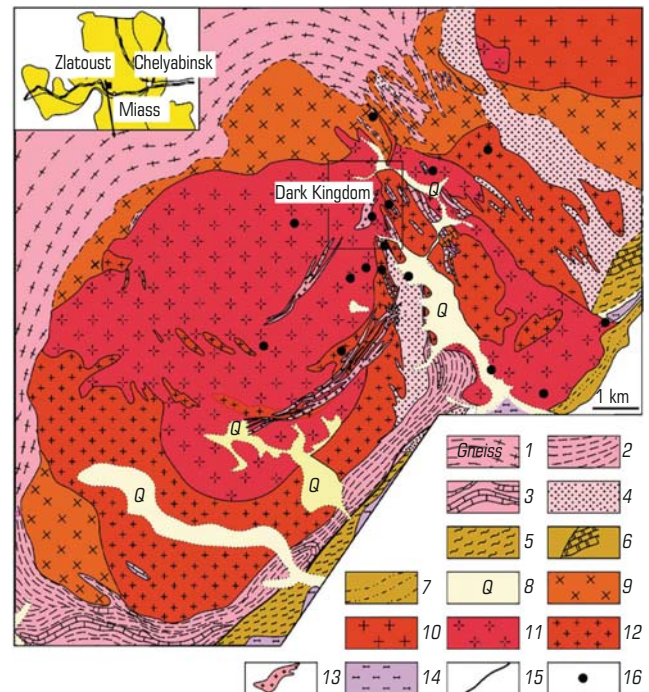
Fig. 1. Geological map of the Syrostan Granite Massif enclosing the Dark Kingdom Marble Deposit ([2] as amended)
